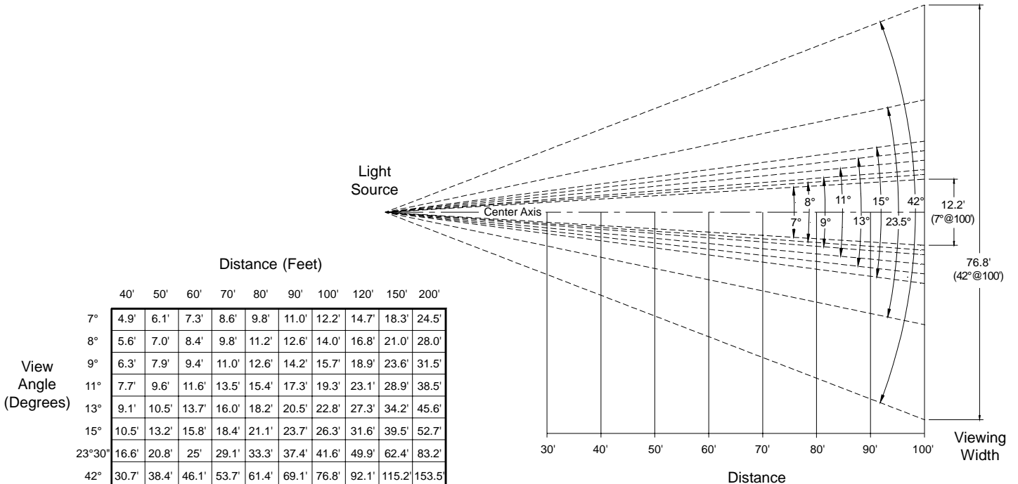
Baffles A thru G (Baffles shown in factory set position for 8°)
